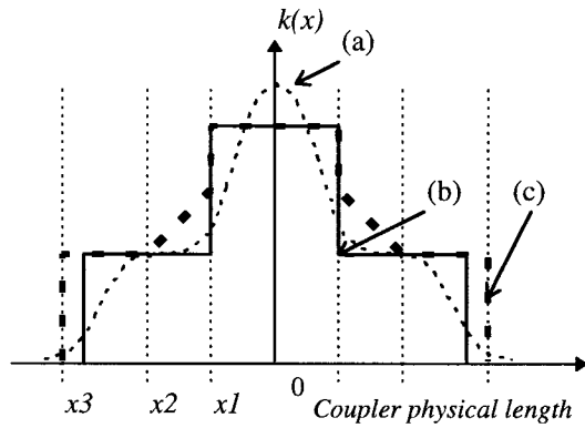
Fig. 1. (a) Coupling distribution for nonuniform line, (b) for multisection line, and (c) for nonuniform line approximation.
