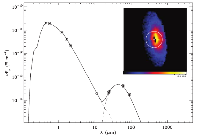
FIG. 4.—Observed SED of HD 15745 along with our best-fitting model (see text for model parameters). Our new N ( \lambda_c = 11.2 \mu\text{m} , \Delta\lambda = 2.4 \mu\text{m} ) Gemini measurement is indicated with a diamond (Gemini program ID GN-2006B-C-12). HD 15745 is unresolved, with a FWHM of 0.3'' in the north-south direction, and 0.5'' in the east-west direction. Photometric calibration was accomplished by observing HD 20893 in N and assuming an extinction of 0.172 \text{ mag per air mass} . The 24\text{--}90 \mu\text{m} data represent the IRAS and ISO values given by Moór et al. (2006). The dotted and dashed curves represent the stellar and disk emission, respectively. The inset is a log-stretch image of our best-fit model, observed with an inclination of 67^\circ and rotated so as to match the orientation of the disk in Fig. 1. The white circle represents the 2'' radius region that is hidden in Figs. 1 and 2.
