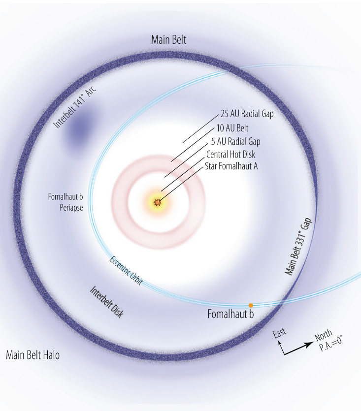
Figure 26. Notional sketch of the Fomalhaut system viewed face-on. The radial locations of features are approximate and not to scale. For example, the 10 AU belt represents dust near 10 AU radius, but the width of the belt is not precisely known.
