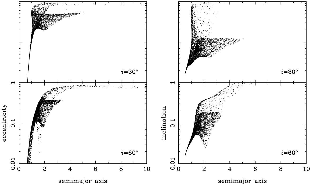
Figure 12. The final eccentricity and inclination against semimajor axis distributions for parabolic fly-by simulations with orbital inclination i = 30^\circ and 60^\circ .
