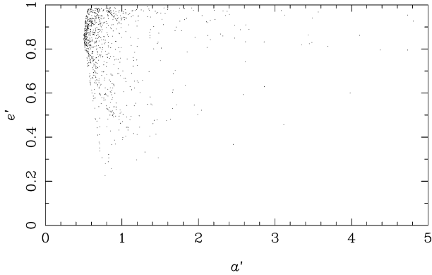
Figure 15. Particle positions and eccentricity versus semimajor axis for captured particles relative to the perturber.
