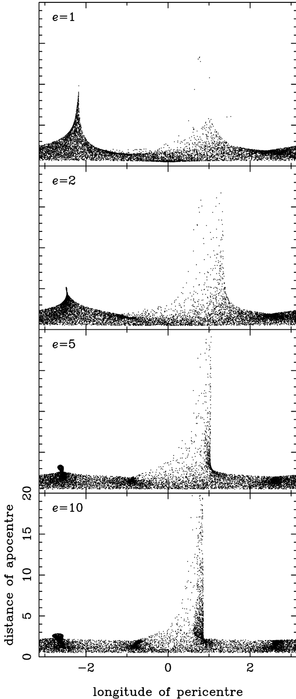
Figure 7. The final distance of apocentre against the longitude of pericentre for fly-by simulations with perturber orbits of eccentricity e = 1, 2, 5 and 10 . Here and in similar plots we select particles with e < 1 and with separations from the secondary of greater than 10 , at the final time level. In all plots involving the longitude of pericentre, zero longitude is defined by the positive horizontal axis in face-on particle position plots.
