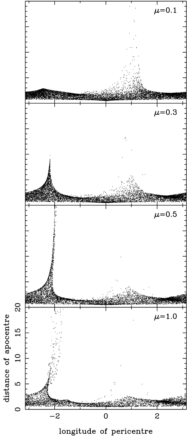
Figure 10. The final apocentre distance against longitude of pericentre distribution for parabolic fly-by simulations with perturber masses of 0.1, 0.3, 0.5 and 1.0 .
