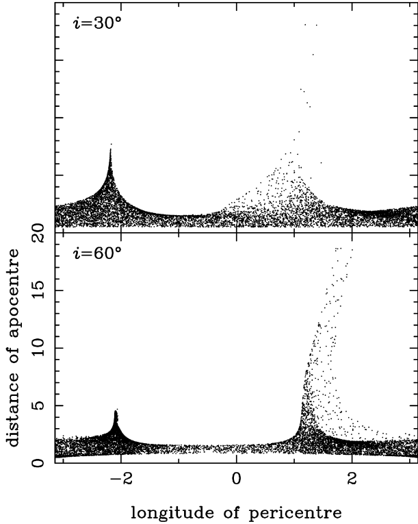
Figure 11. The final distance of apocentre against the longitude of pericentre for parabolic fly-by simulations with orbital inclination i = 30^\circ and 60^\circ .
