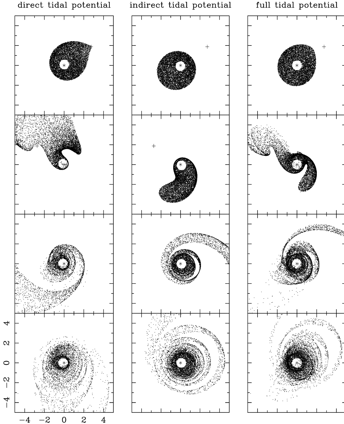
Figure 4. Particle positions at various times for parabolic fly-by encounter simulations that use different components of the tidal potential. From the top row of frames to the bottom the times given are -3 , +3 , +20 and +60 . The perturber is plotted with a cross, and the primary star (origin) is plotted with an asterisk. In these simulations we used \epsilon = 10^{-7} , R_p = 0.1 and R_s = 0.05 and removed particles that went beyond radii greater than 10 from the primary.
