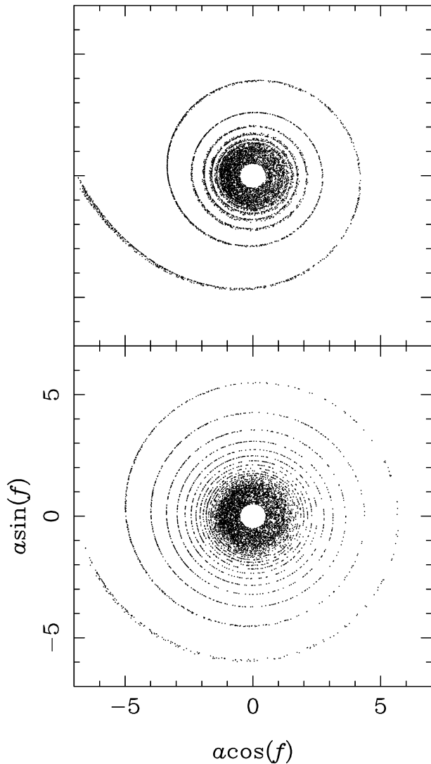
Figure 5. Data for the model using only the indirect component of the tidal potential (see Fig. 4). The top frame is for data taken at a time of +60; the bottom frame corresponds to a time of +180. Plotted are a \cos f against a \sin f for each particle, where a is the semimajor axis and f is the true anomaly.
