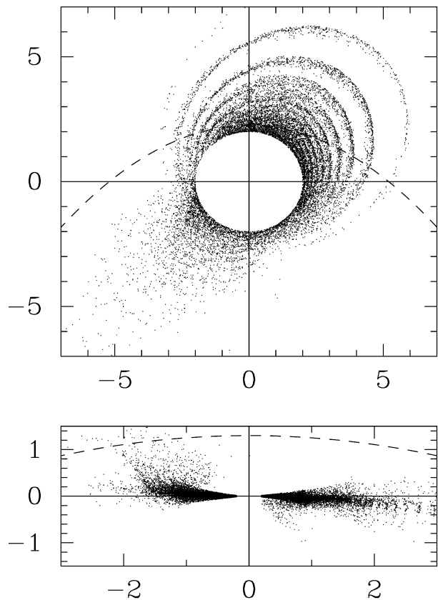
Figure 3. The face-on and edge-on views of a sample of simulation particles in the computational frame centred on the primary mass (labelled fig. 2 in KLSS). The primary is of unit mass and G = 1 , giving a time unit such that the circular orbit period at unit radius is 2\pi . The horizontal axes correspond to the line of nodes of the perturber’s orbit. Parameters are: perturber mass of 0.3, parabolic pericentre distance of 2.6, pericentre inclination of 30^\circ . The disc of \sim 10^6 particles is initially distributed between 0.2 and 2 radius units. The initial vertical density is exponentially decreasing, with an outer height of 0.6, and the aspect ratio and the radial surface density follow radial power laws of index -1.5 . A random sample of \sim 25 per cent of the particles outside the initial radius are shown in the top frame, the bottom frame shows a thin slice of particles about the horizontal axis. The path of the perturber is indicated with a dashed line and it enters the frame from the right-hand side. The positions and velocities of the particles are integrated with a second-order leapfrog scheme; the perturber orbit is prescribed as a function of time. The configuration shown is for a time of 160 units after pericentre passage. The perturber was introduced at a separation from the primary of 20 units.
