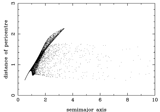
Figure 14. The final eccentricity and distance of pericentre against semimajor axis for a hyperbolic fly-by simulation with orbital eccentricity e = 2 and orbital inclination i = 30^\circ .
