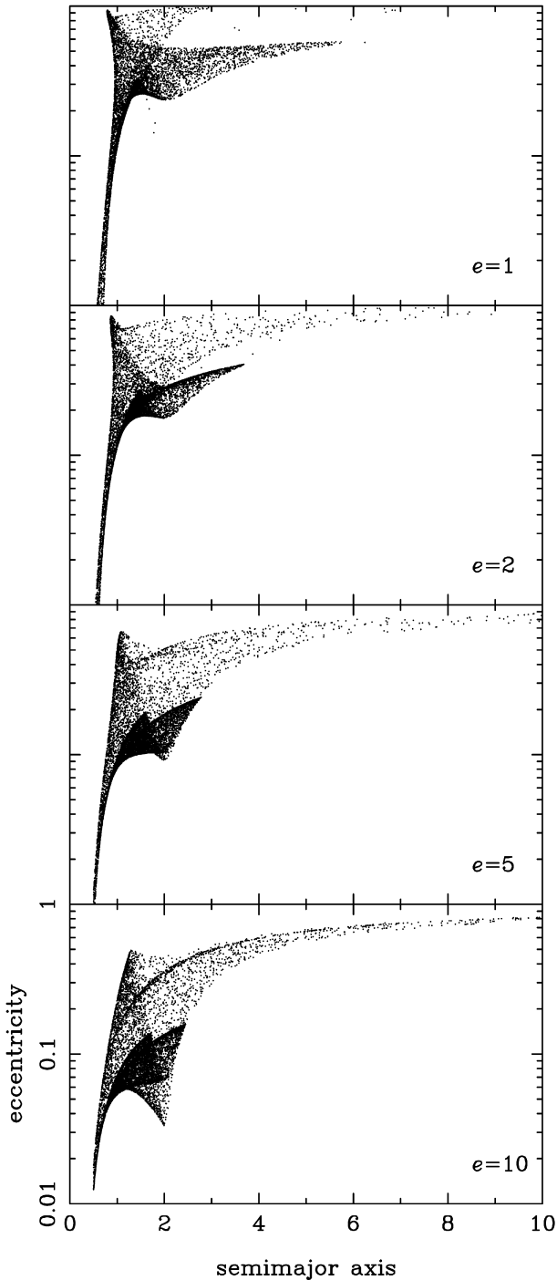
Figure 9. The final eccentricity against semimajor axis distribution for fly-by simulations with perturber orbits of eccentricity e = 1, 2, 5 and 10 .
