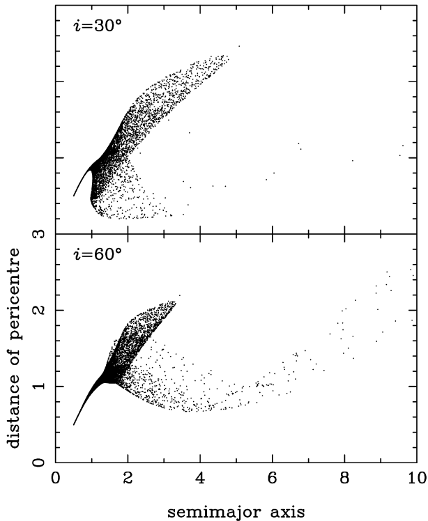
Figure 13. The final distance of pericentre against semimajor axis for parabolic fly-by simulations with orbital inclination i = 30^\circ and 60^\circ .
