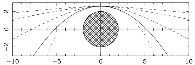
Figure 6. Schematic representation of the initial disc (cross-hatched circle), and the orbital paths of a perturber for a parabolic encounter (solid line) and hyperbolic encounters (dashed lines, from lowermost to uppermost, for e = 2, 5 and 10 respectively). The dotted line corresponds to a bound orbit with e = 0.75 (see Section 3.5). As for the simulations, the origin is assumed to be fixed to the primary.
