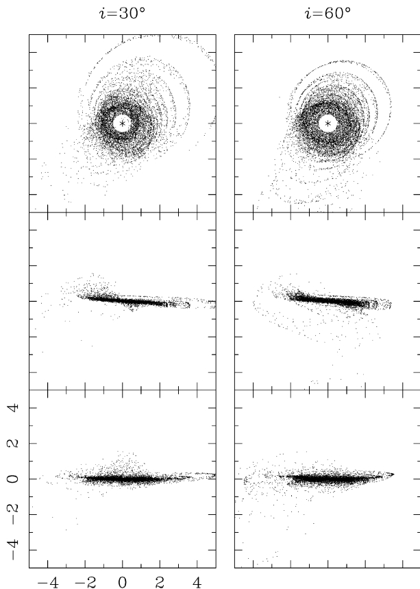
Figure 19. Summary of inclined-orbit models in face-on and edge-on particle plots. The models were run for 120 time units, with the perturber initialized a radial distance of 20 from the primary. The left-hand panel shows results for the model with e = 1 , \mu = 0.3 and i = 30^\circ . The right-hand panel shows results for the corresponding case with i = 60^\circ . Uppermost frames are face-on views, middle frames are edge-on projections along the horizontal axis (line of nodes), and bottom frames are edge-on projections along the axis defining i = 0 . Thus the projections are on to the three mutually orthogonal Cartesian planes of the computational coordinate system. The position of the primary is plotted with an asterisk.
