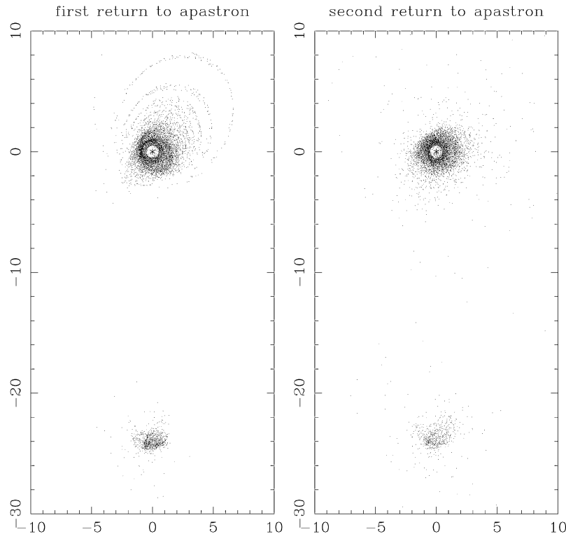
Figure 17. Particle positions corresponding to data given in Fig. 16. The position of the primary is plotted with an asterisk.
