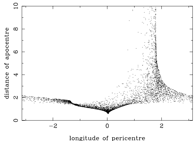
Figure 8. The final distance of apocentre against the longitude of pericentre for a fly-by simulation with a parabolic perturber orbit in which only the direct tidal potential has been used. Data correspond to those given in Fig. 4.
