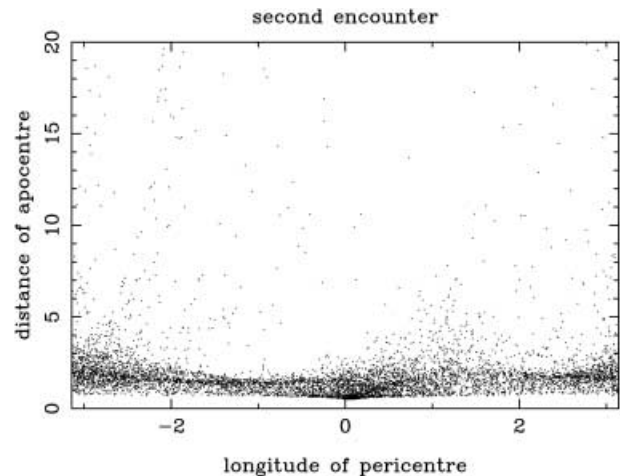
Figure 16. The final distance of apocentre against the longitude of pericentre for a bound orbit fly-by simulation with e = 0.8 . The companion starts at apocentre and was set up and integrated much as for the hyperbolic orbit cases. Data are given for the first and second complete orbits. In this simulation we used \epsilon = 10^{-7} .
