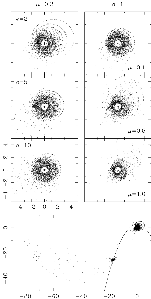
Figure 18. Summary of coplanar model results in face-on particle plots. The models were run for 120 time units, with the perturber initialized a radial distance of 20 units from the primary. After much longer times the phase mixing in the particles' orbits results in dissolution of the ring features, maintaining the distended envelopes of the discs seen above. The position of the primary is plotted with an asterisk. The top left-hand side panel shows results for models with \mu = 0.3 and from top to bottom e = 2, 5 and 10 respectively. The top right-hand side panel shows results for models with e = 1 and from top to bottom \mu = 0.1, 0.5 and 1 respectively. The bottom panel shows results, on a larger scale, for the model with e = 1 and \mu = 0.3 . The perturber trajectory is shown with a solid line. We see: the perturbed disc with rings, the captured particles clustered about the instantaneous position of the perturber, and escaping particles (the large arcs on the left-hand side of the plot).
