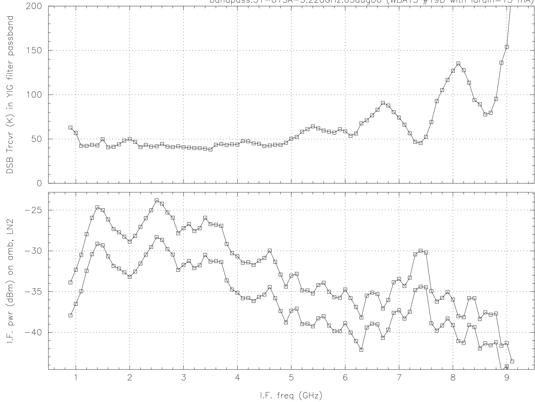
bandpass.31-015A-5.220GHz.03aug06 (WBA13 #19D with Idrain=13 mA)
