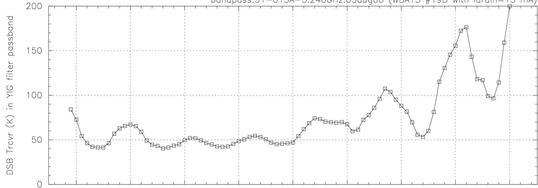
bandpass.31-015A-5.240GHz.03aug06 (WBA13 #19D with Idrain=13 mA)
