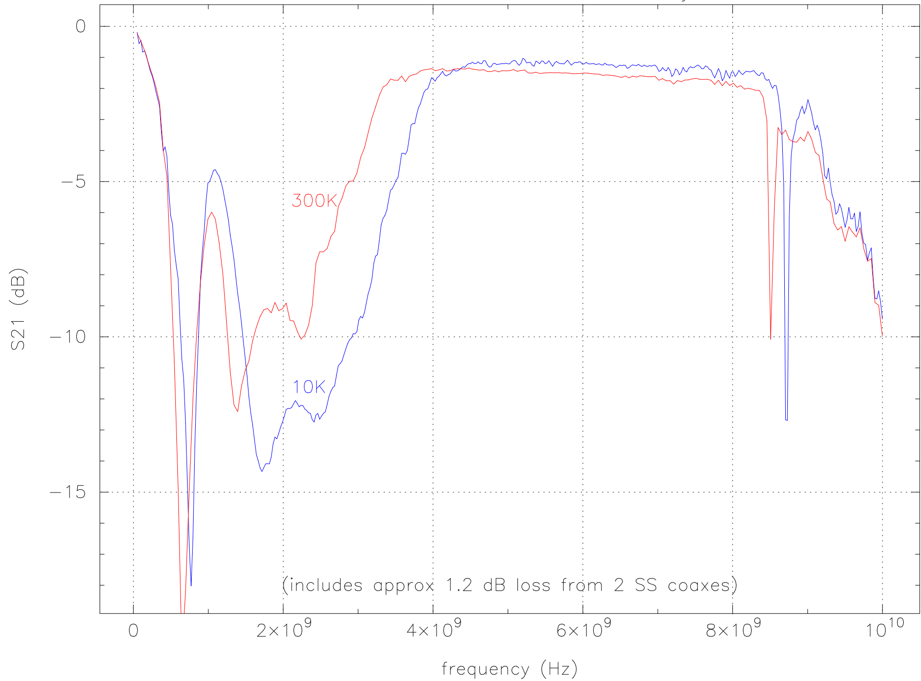
Trak 4-8 circulator tested in 350 dewar, 17jan2007
