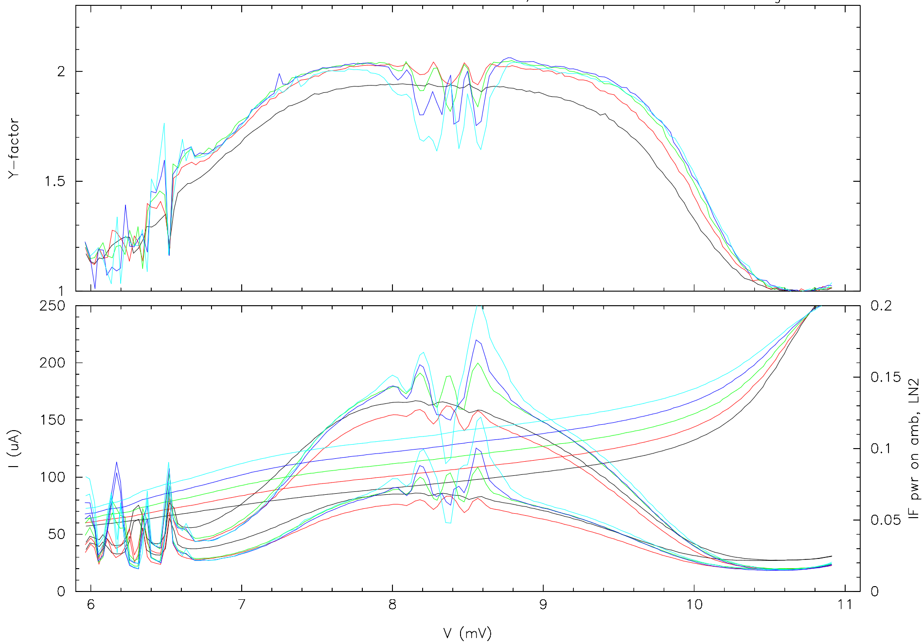
mixer 31-042-03; scans at 250 GHz with 0 mA magnet current
