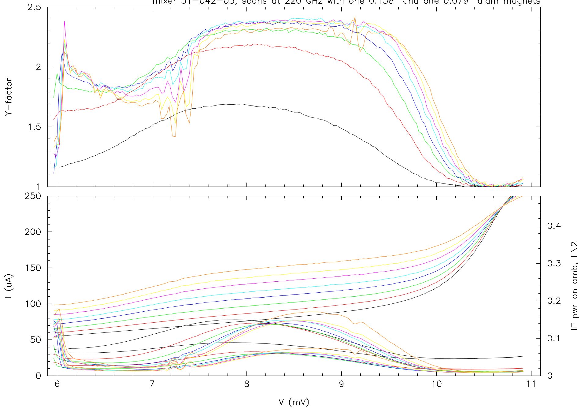
mixer 31-042-03; scans at 220 GHz with one 0.158" and one 0.079" diam magnets
