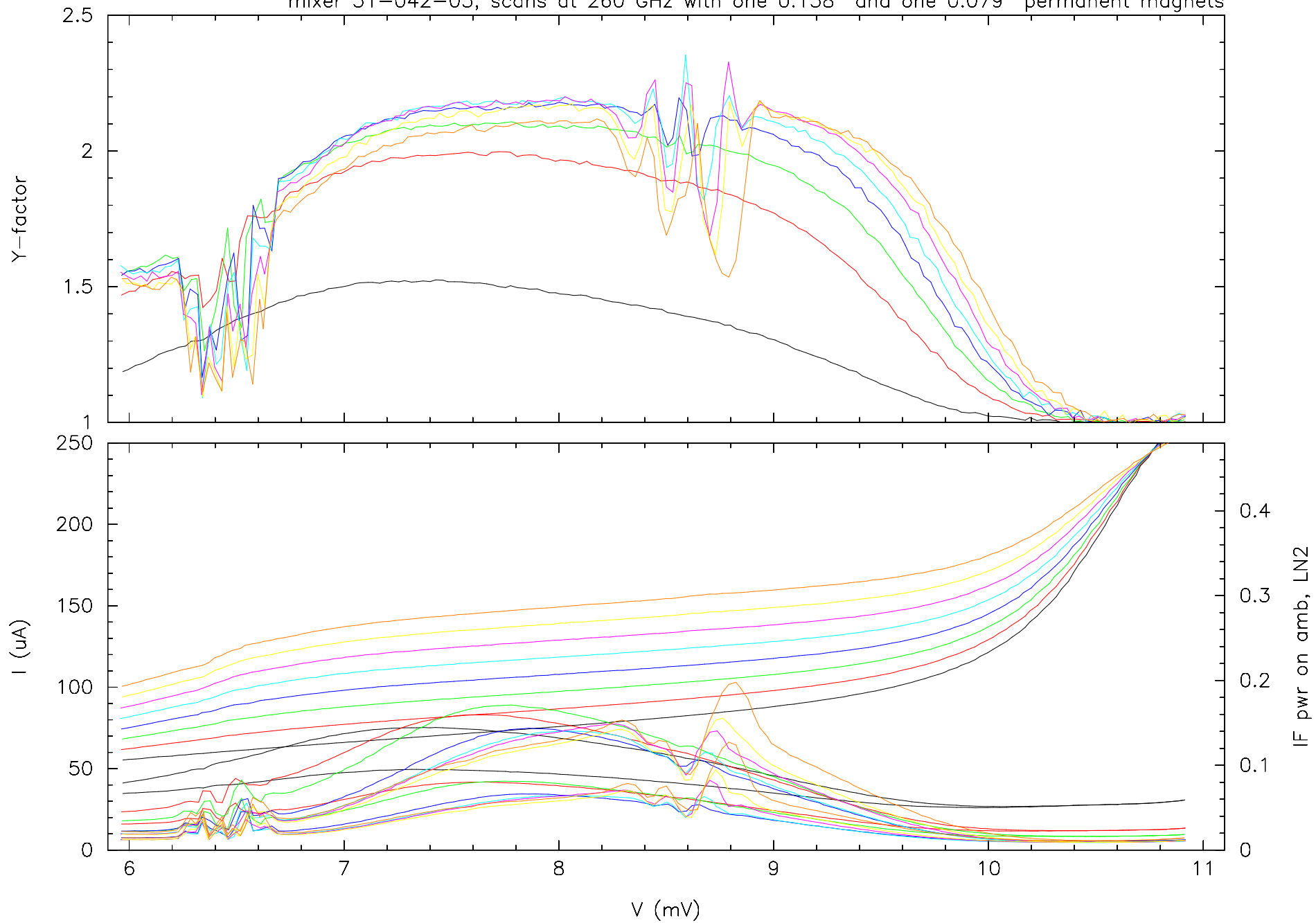
mixer 31-042-03; scans at 260 GHz with one 0.158" and one 0.079" permanent magnets
