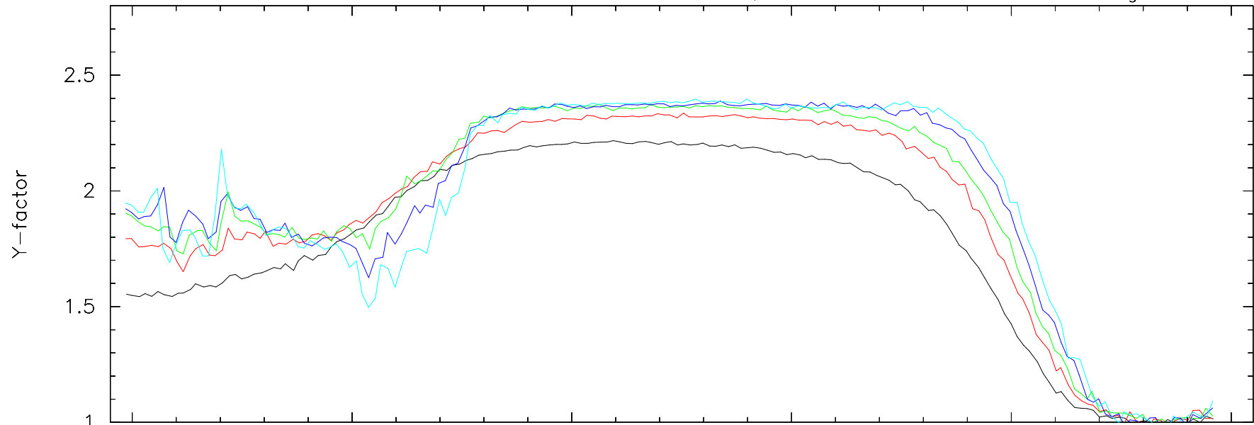
mixer 31-042-03; scans at 220 GHz with 45 mA magnet current
