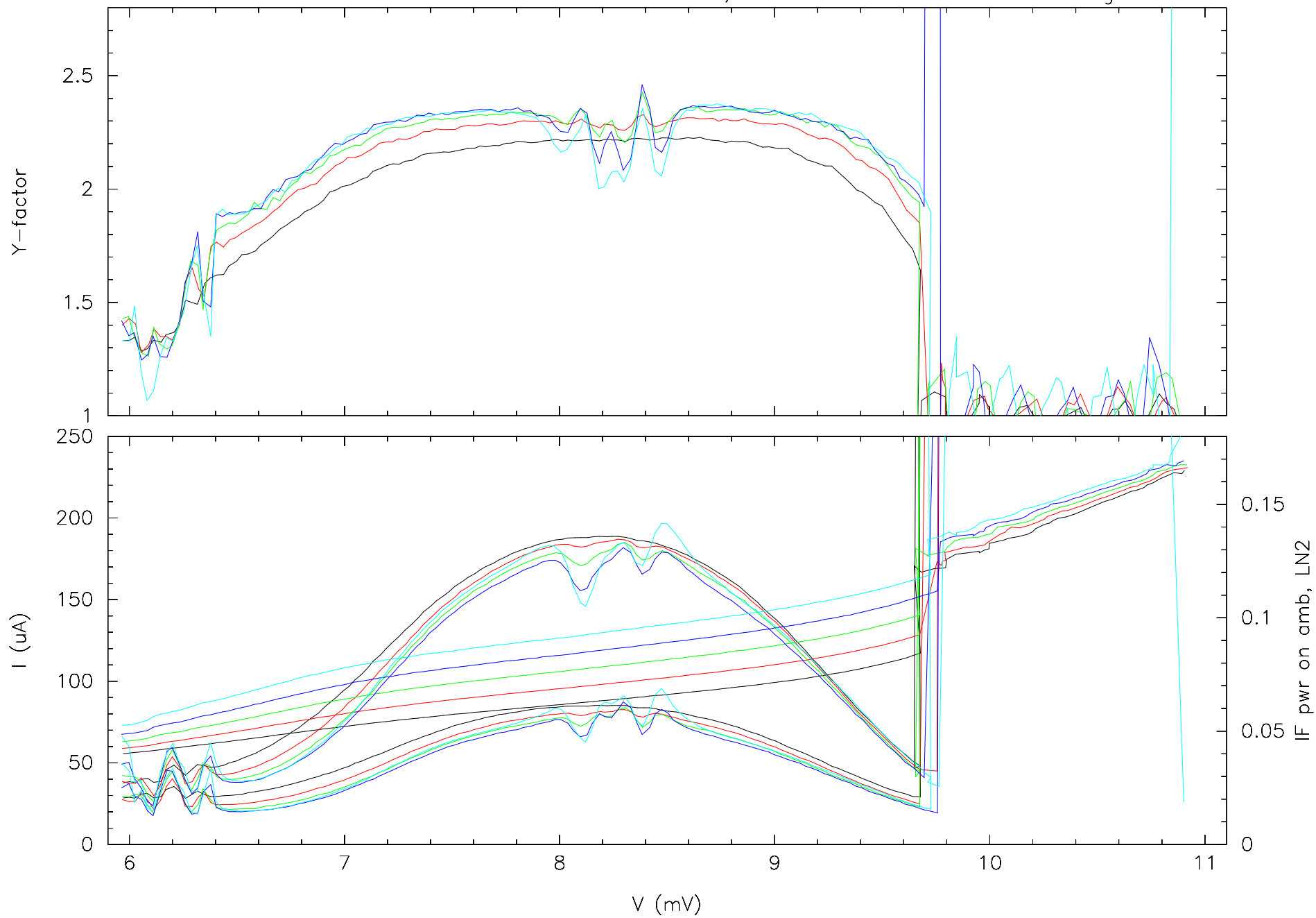
mixer 31-042-05; scans at 250 GHz with 135 mA magnet current
