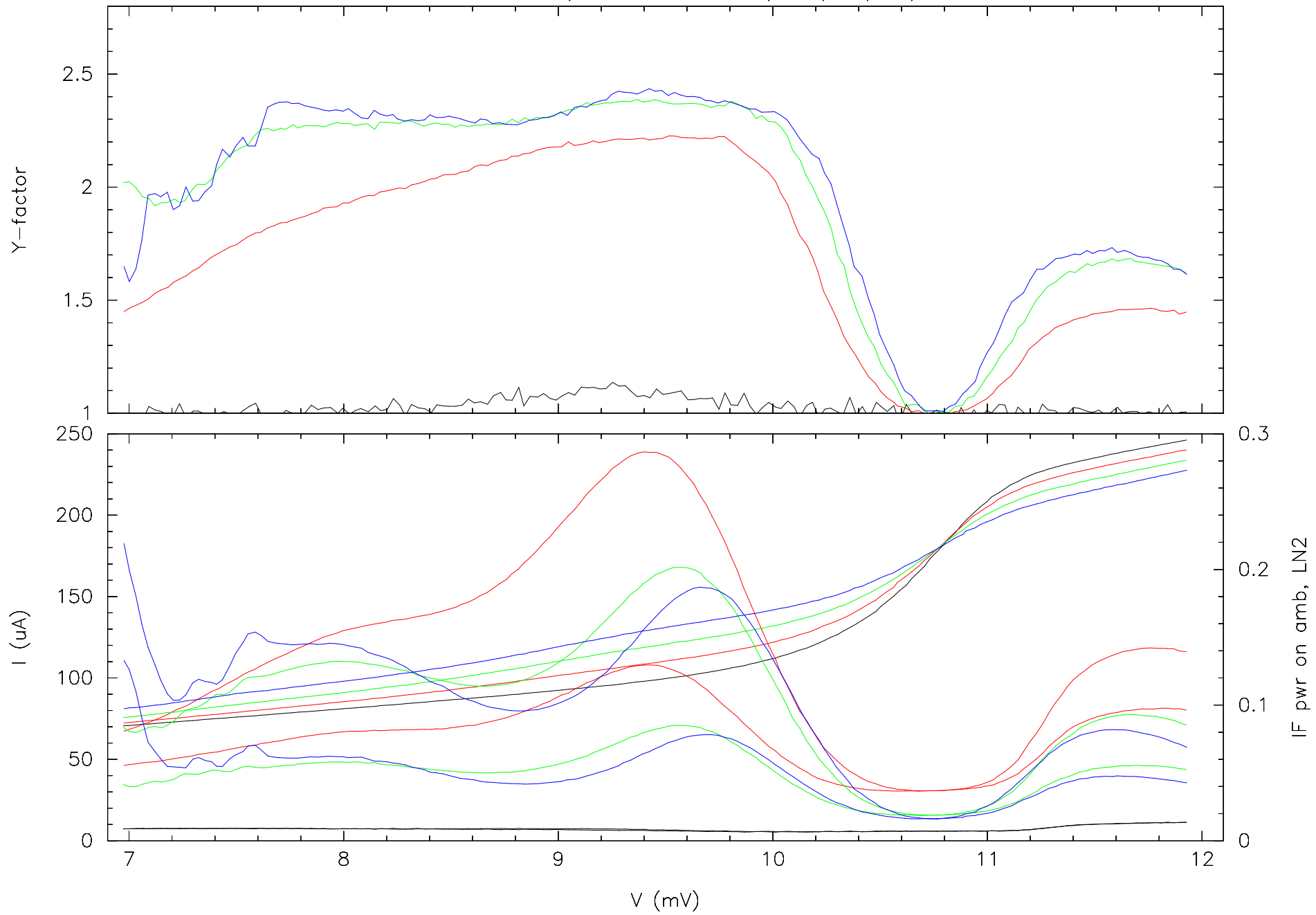
mixer HIA-091; scans at 110 GHz; 110,120,130,140 uA bias current at 10 mV
