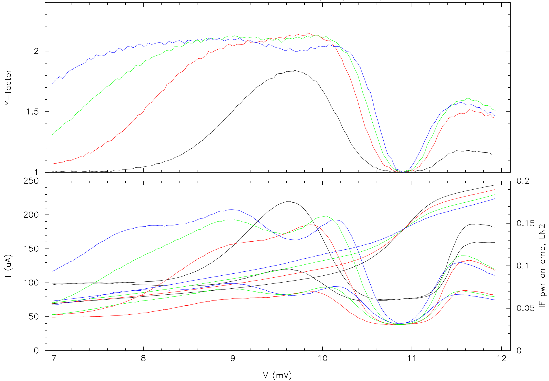
mixer HIA-091; scans at 77 GHz; 110,120,130,140 uA bias current at 10 mV
