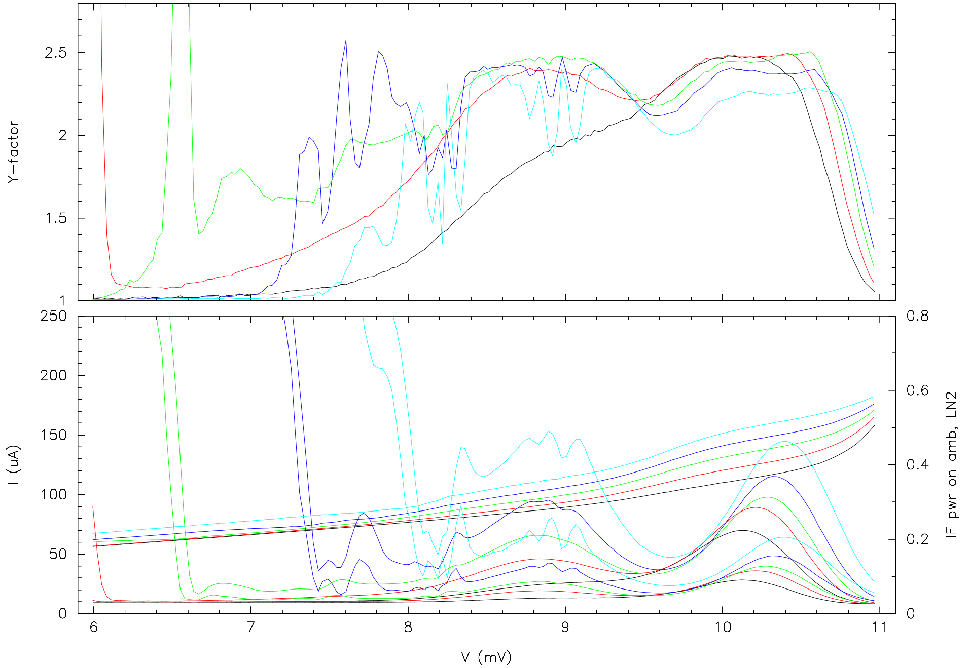
mixer HIA-173; scans at 90 GHz; bias 110,120,130,140,150 \mu\text{A}
