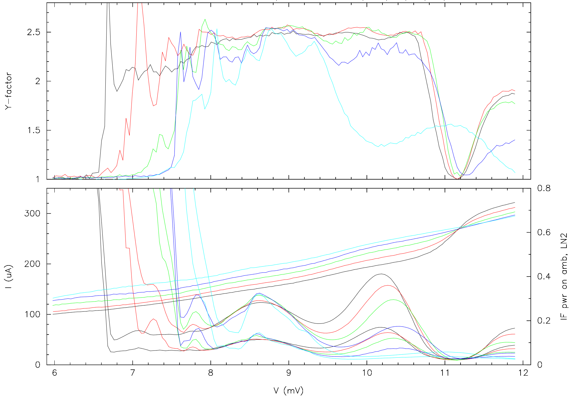
mixer HIA-180; scans at 100 GHz; 160,170,180,190,200 \mu\text{A} at 10.2 mV
