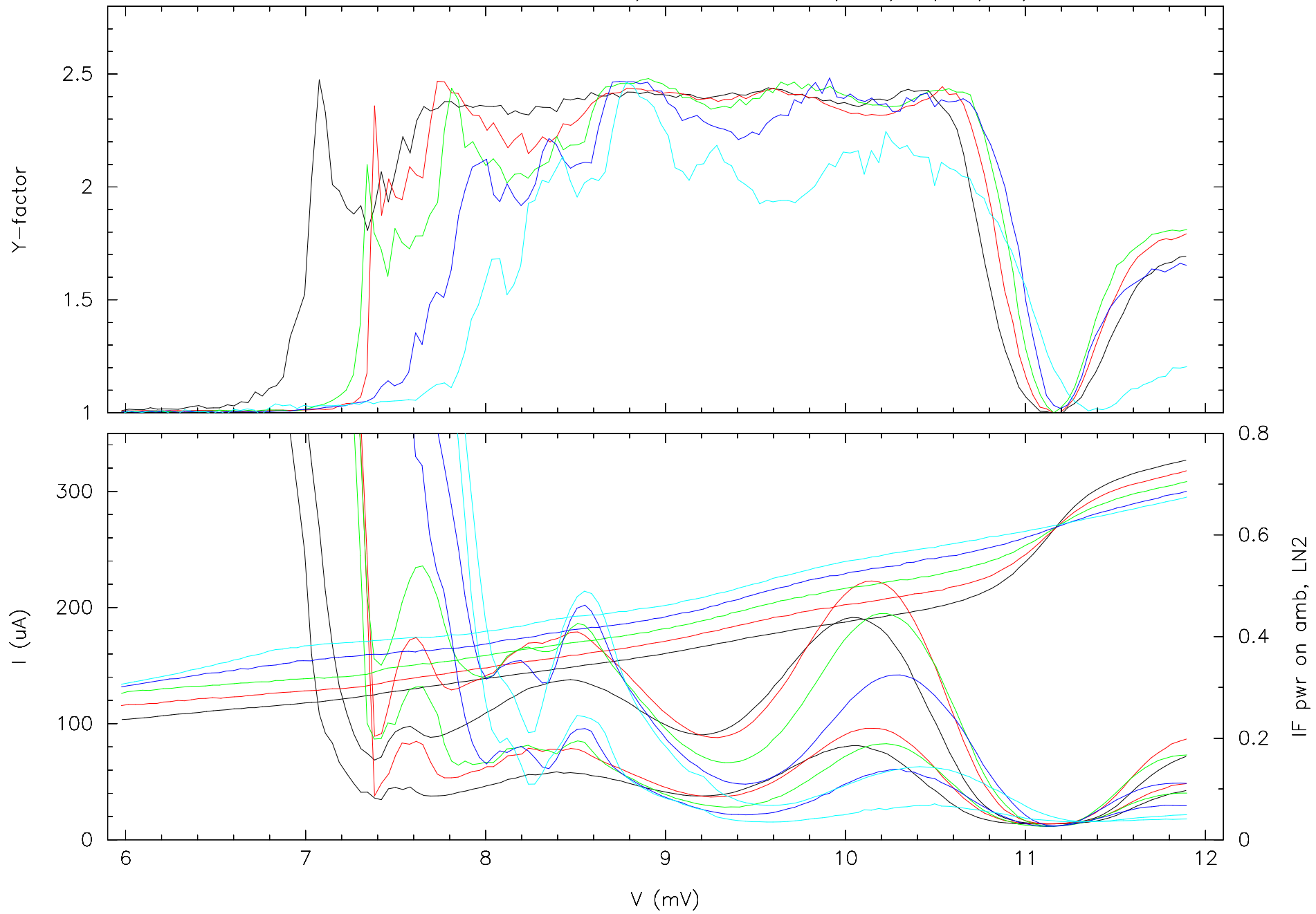
mixer HIA-180; scans at 110 GHz; 160,170,180,190,200 uA at 10.2 mV
