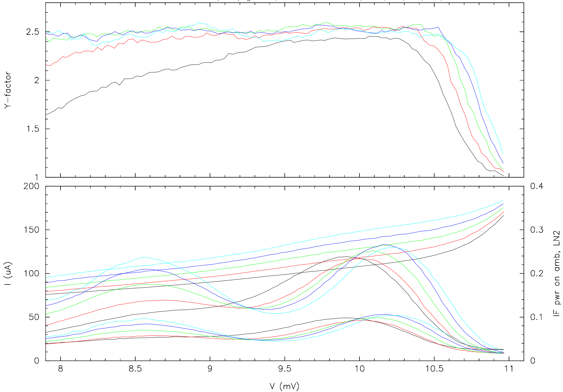
mixer HIA-188, amp #131D, scans at 100 GHz; 110,120,130,140,150 \mu\text{A} at 10.1 \mu\text{A}
