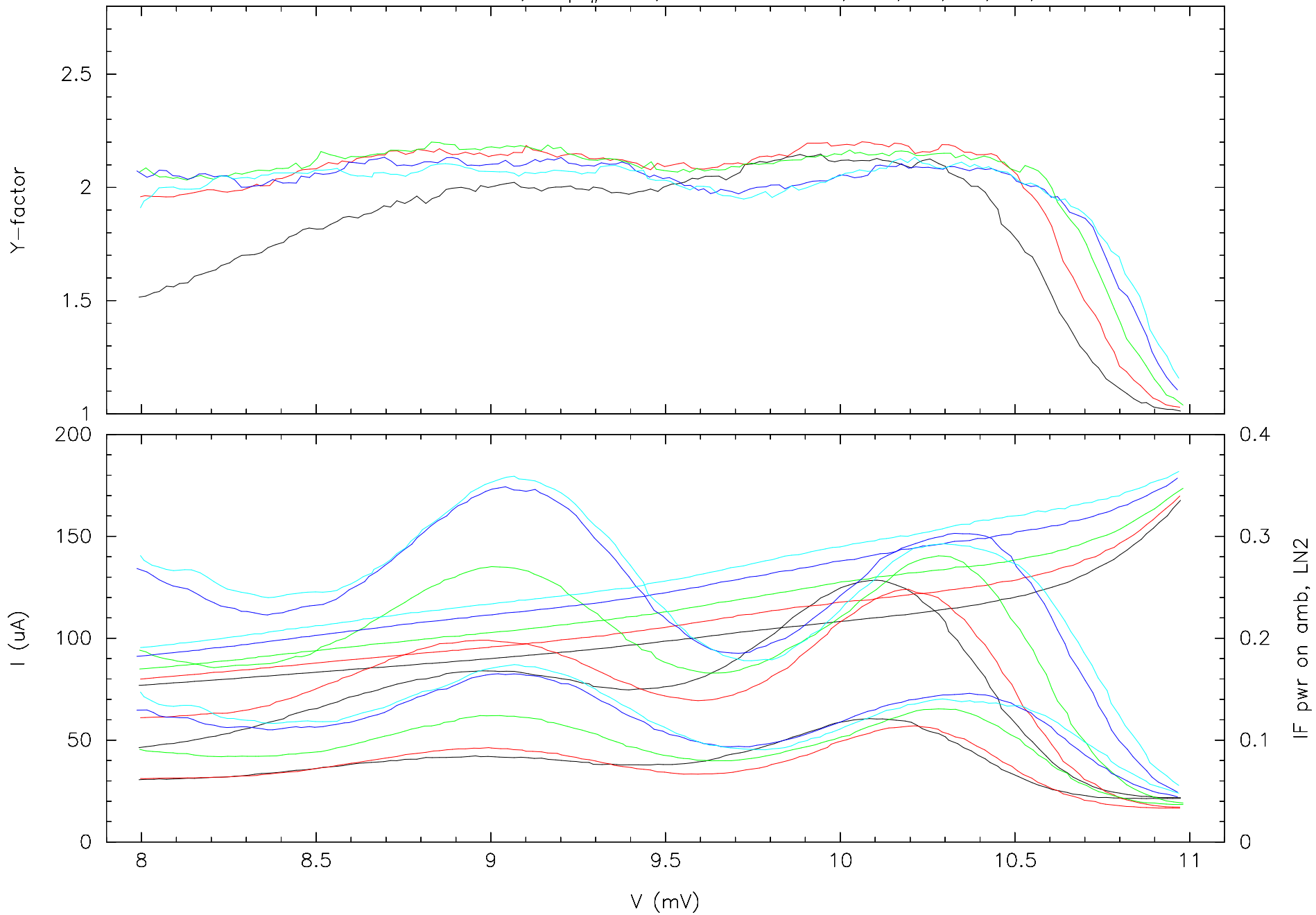
mixer HIA-188, amp #131D, scans at 80 GHz; 110,120,130,140,150 uA at 10.1 uA
