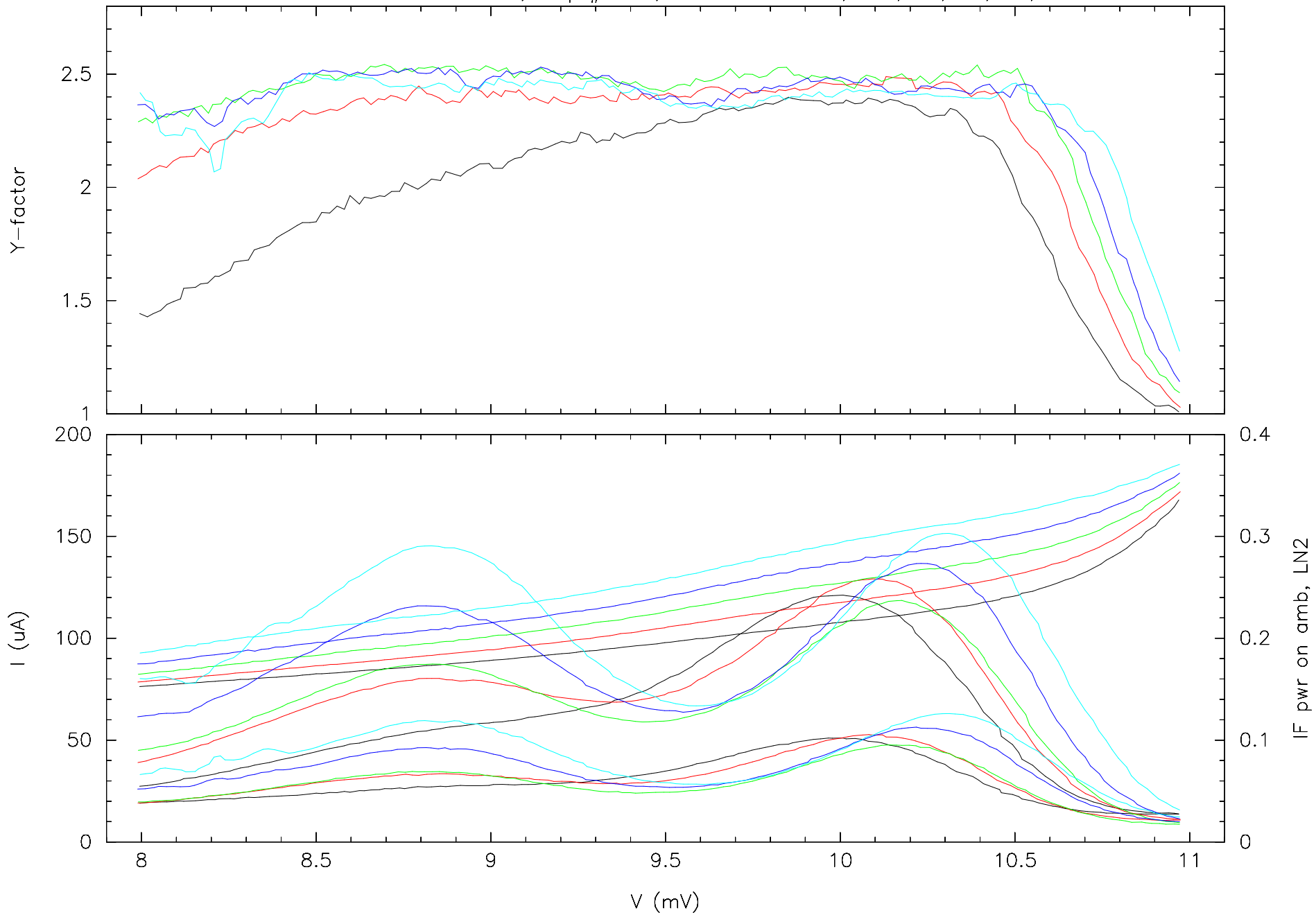
mixer HIA-188, amp #131D, scans at 90 GHz; 110,120,130,140,150 \mu\text{A} at 10.1 \mu\text{A}
